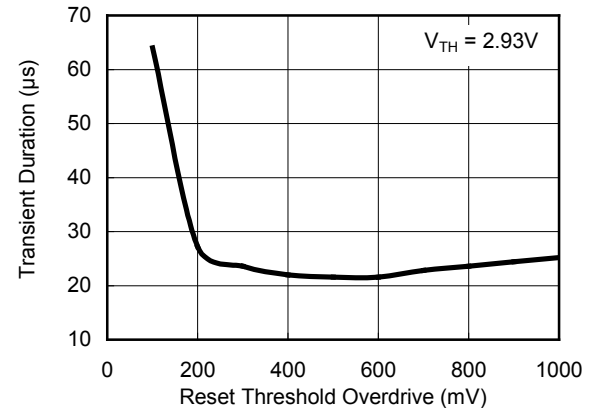
Maximum Transient Duration vs. Reset Threshold Overdrive
