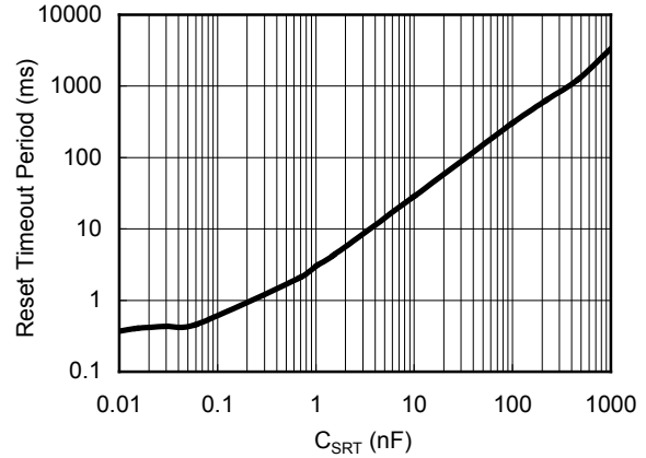
Reset Timeout Period vs. C_{SRT}
