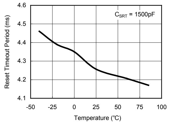
Reset Timeout Period vs. Temperature
