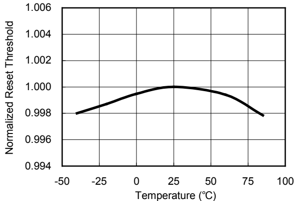
Normalized Reset Threshold vs. Temperature
