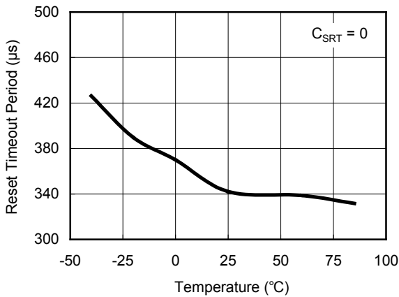
Reset Timeout Period vs. Temperature
