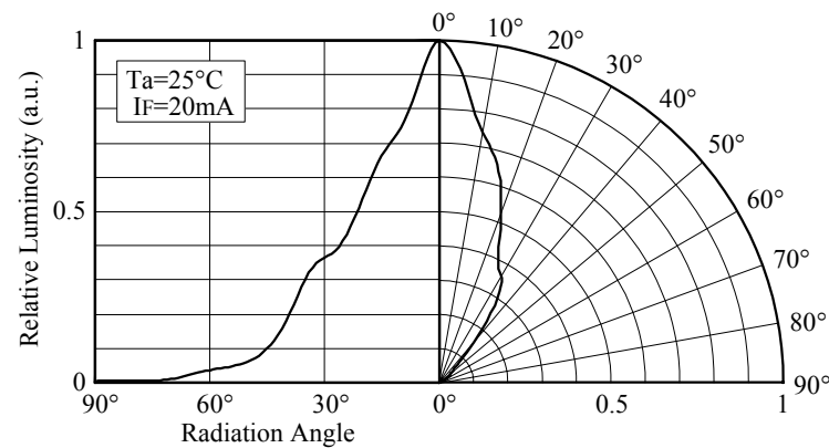
■ Directivity (NSPB520S)
